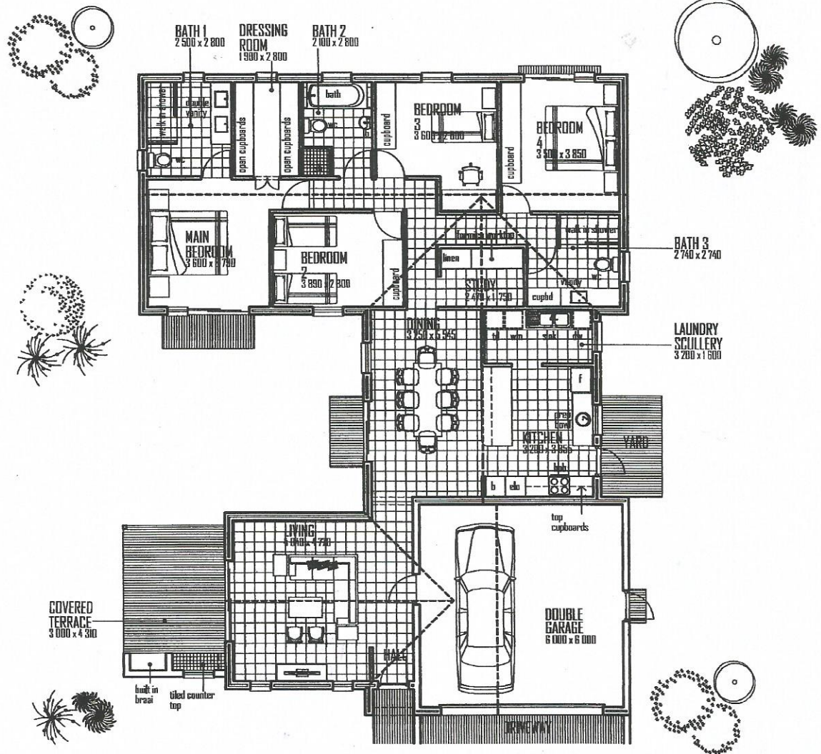
FLOOR PLAN
